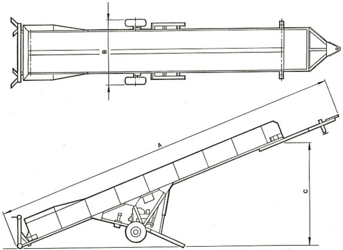
AQUAMARINE SC130 & SC-230 SHORE CONVEYORS
